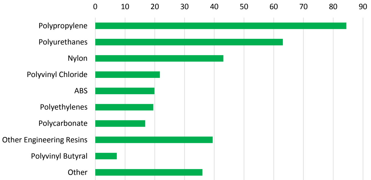
Figure 3 Average Plastics & Polymer Composites Use in North American (NAFTA) Light Vehicles in 2018 (pounds/vehicle)
